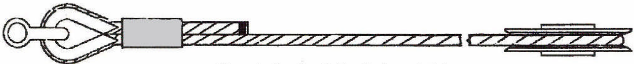
Figure 2: Pendant Cable with Swaged Ends (New Style)
